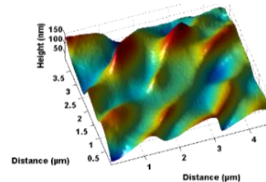
Figure 3: Nanoripples on stainless steel measured with microsphere-assisted WLSI [3].
